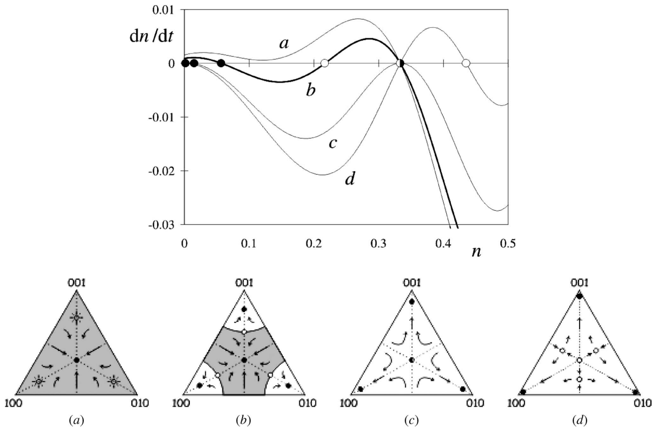
Figure 8. The rate of change dn/dt as function of n along the three symmetry axes of the three-compartment system (see Equation (15)), for four successive values of B : (a) B = 0.72 , (b) B = 0.78 , (c) B = 1.0 , and (d) B = 1.56 . For each of these values a triangular flow diagram is given, which shows the dynamics of the full system. The shaded area is the (diminishing) basin of attraction of the uniform equilibrium \{\frac{1}{3}, \frac{1}{3}, \frac{1}{3}\} in the centre of the triangle; the white regions are the basins of attraction of the clustered solutions. Closed circles represent stable equilibria, open circles unstable ones. From [59]. Reprinted from Europhys Lett. , 53, 328 (2001). Copyright 2001 by EDP Sciences.
